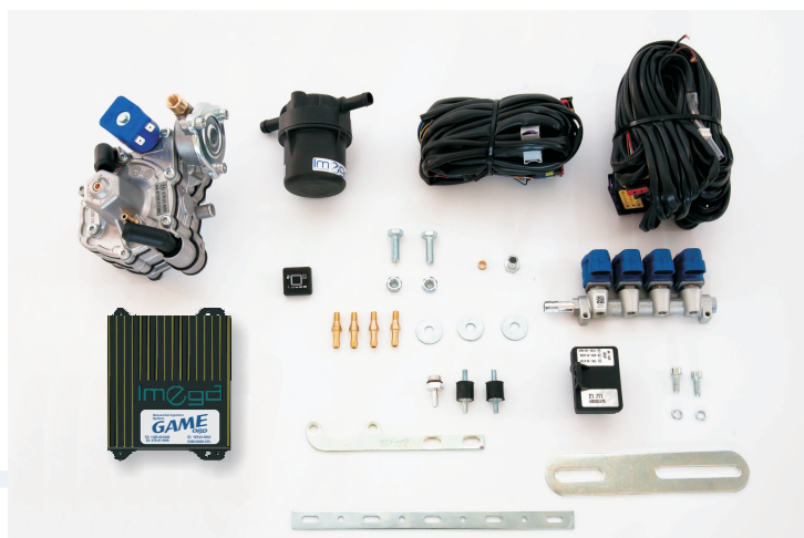
Kit Imega Game OBD LPG
