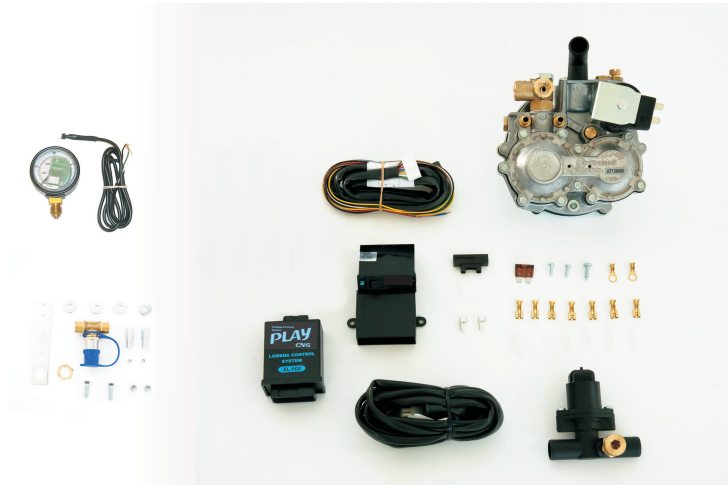
Kit Imega Play CNG
